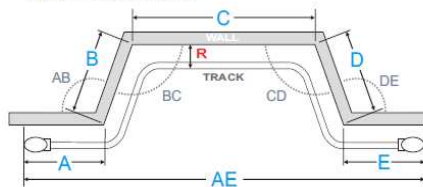
Style 4 Measurements
