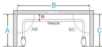
Style 3 Measurements
