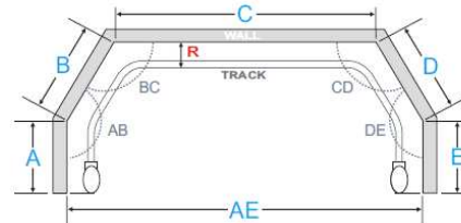
Style 4 Measurements
