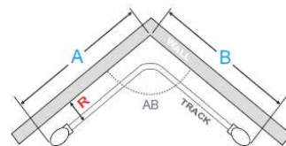
Style 5 Measurements
