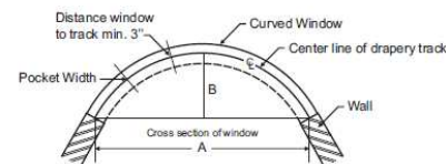
Figure 3: Critical Dimensions of a Curved Track
