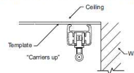
Figure 2: Template on the Ceiling Facing Down
